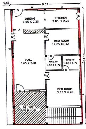
PROP. FIRST FLOOR PLAN SCALE 1:100
