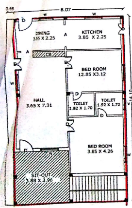
PROP. GROUND FLOOR PLAN SCALE 1:100
