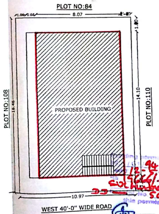
PLAN & SITE PLAN SCALE 1:200
