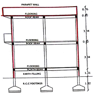
SECTION AT - XX
