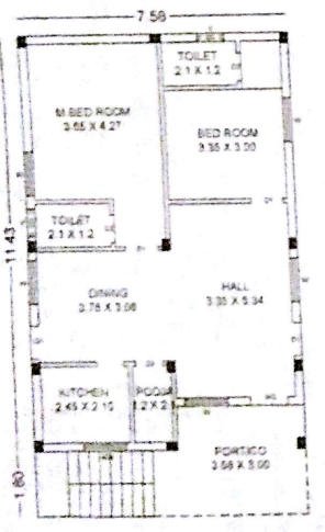
PROP. GROUND FLOOR PLAN
