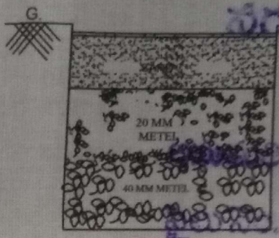
C/S OF RWH PIT
