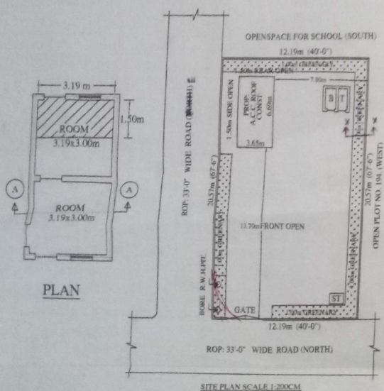
SITE PLAN SCALE 1:200CM
