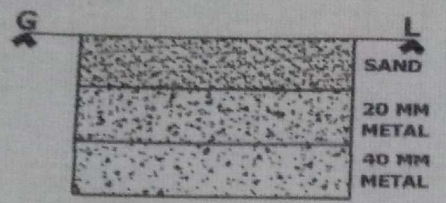
CROSS SECTION OF RAIN WATER HARVESTING PIT
