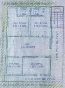
EXIST GROUND FLOOR PLAN
