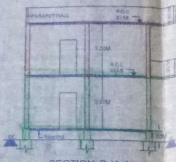
SECTION @ 1A-1'
