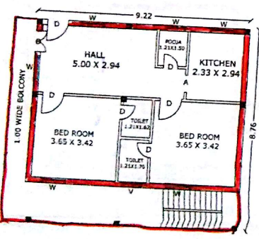
PROP: GROUND FLOOR PLAN
