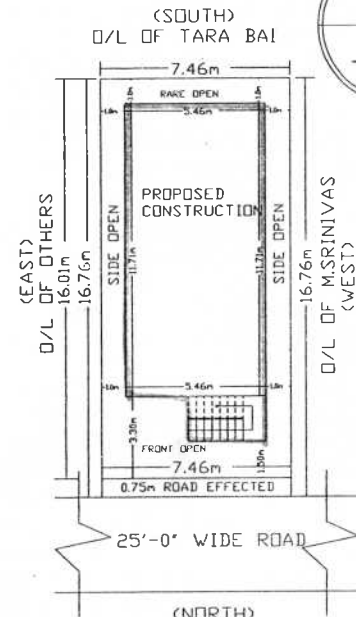
(NORTH) SITE PLAN
