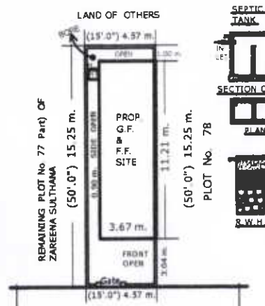
SITE- PLAN SCALE : 1:200 cm.
