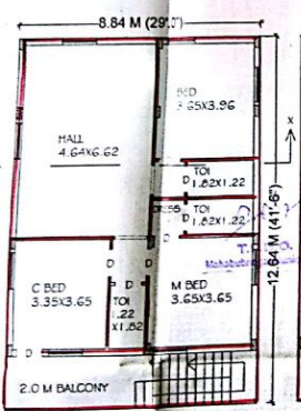
PROPOSED FIRST FLOOR PLAN
