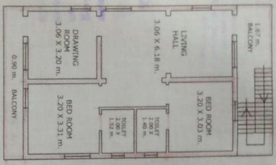
PROP. F. FLOOR PLAN
