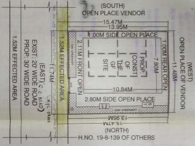
SITE PLAN SCALE 1:200CM
