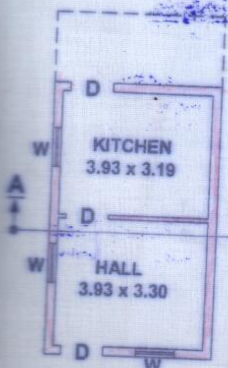
G.F. PLAN
