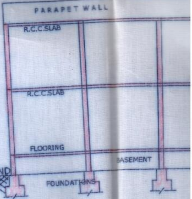
SECTION ON 043
