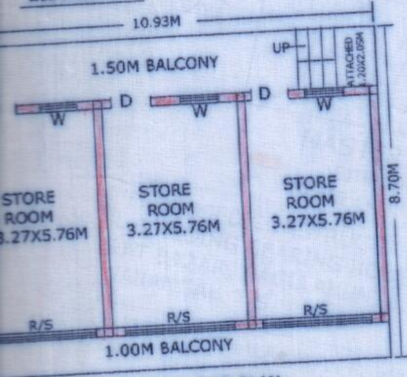
PROP. FIRST FLOOR PLAN
