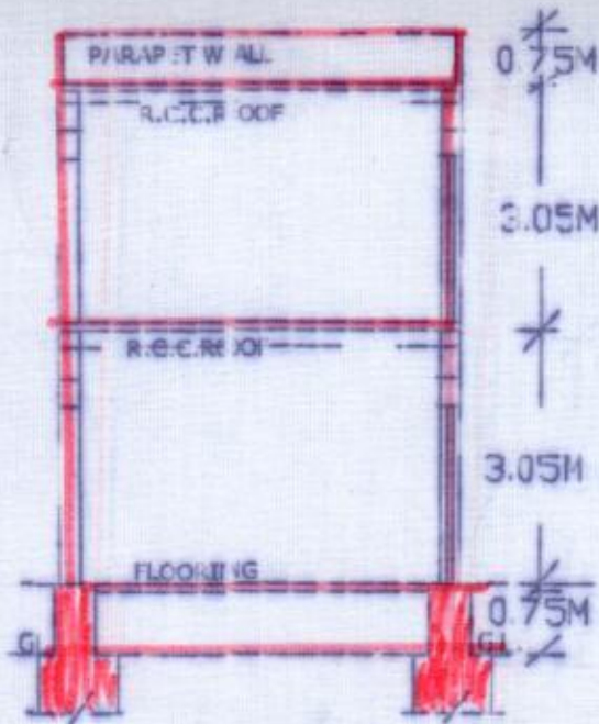
SECTION ON S.S.
