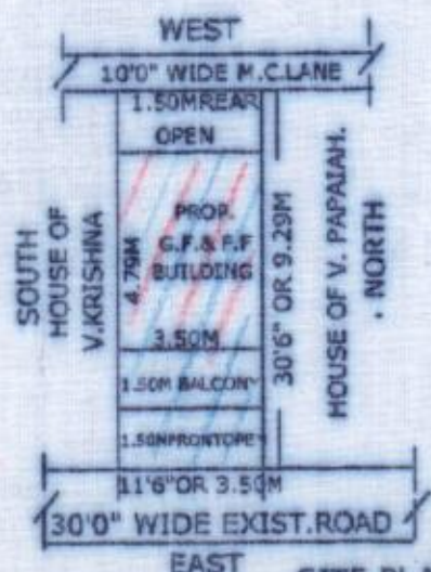
SITE PLAN SCALE 1:200CM
