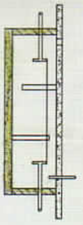
SECTIONAL ELEVATION
