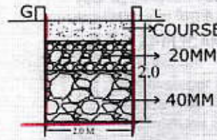
SECTIONAL ELEVATION
