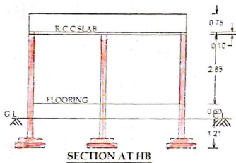
SECTION AT 'HB'
