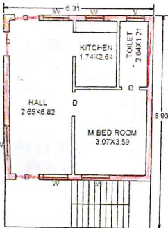
PROP.GROUND FLOOR PLAN
