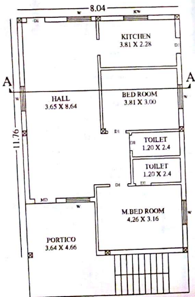
PROP. GROUND FLOOR PLAN
