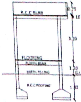
SECTION AT-AA
